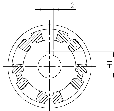
MOTOR SIDE
